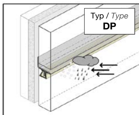
Fugenprofil horizontal Horizontal seal joint
