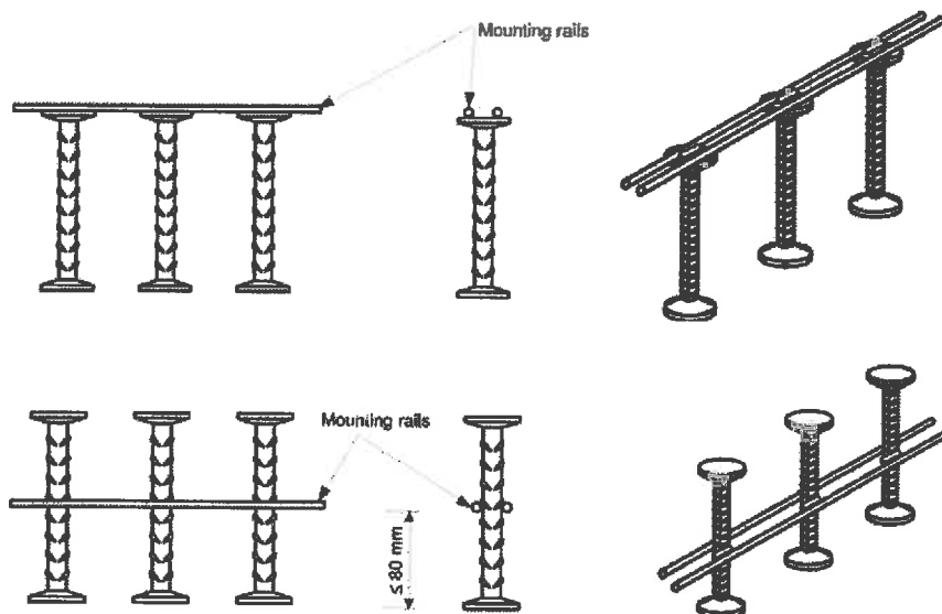
Figure 1: ANCOPLUS double headed studs with mounting rails welded to the head or to the shaft
