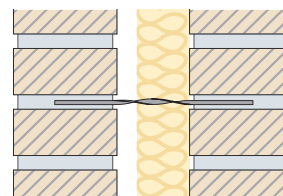
MX-Spiral Anchor
