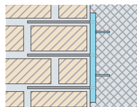
XMS-Masonry Tie Bar
