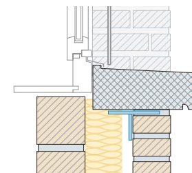
FBK Windowsill Brackets
