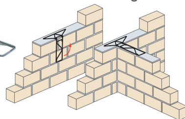
KLP -Folding Anchor
